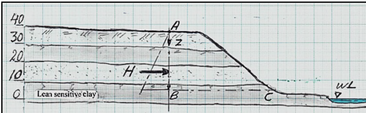
Figure 4.4. Typical slope section close to the 2014 landslide between Goose Bay and Muskrat Falls. This section is assumed to have marine sediments similar to those in the North Spur.
